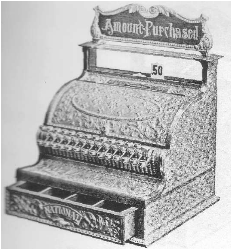
No. 40 Total-Adding Cash Register. Dimensions: 16 1/2 inches wide, 16 inches deep, 22 inches high.
