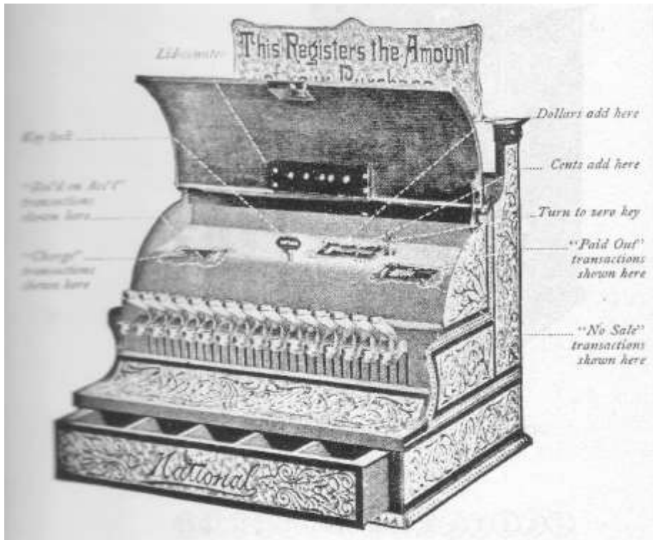
Diagram showing the adding mechanism of the No. 35 National Cash Register.
