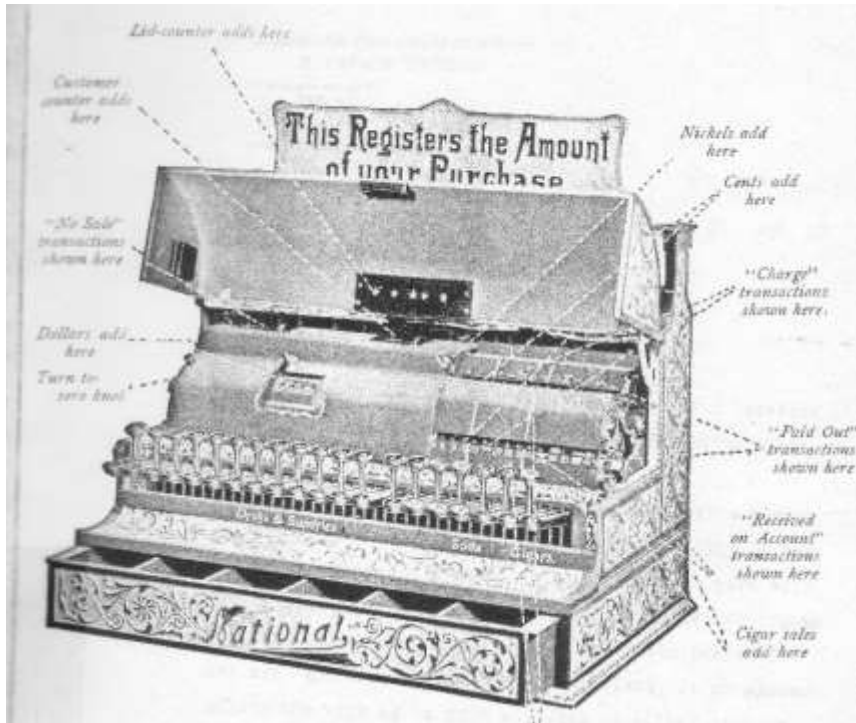
Diagram showing the adding mechanism of the No. 64 National Cash Register.
